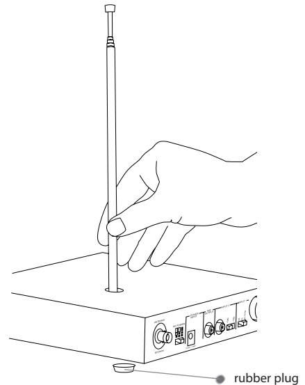
LT-800 shown with top mount antenna connected through top of unit (part numbers LA-101, LA-106 (72 MHz) or LA-102 (216 MHz))
